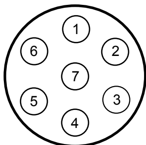
ISO 1724 7-pol
